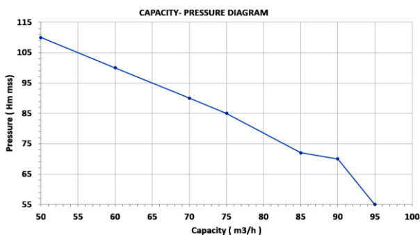
P014- 45D - KP65B3/50 P015 - 45 HP Diesel Motopump Water Cooler - 4 Cylinders 3 Stage High Pressure with Trailer Suction 4" - Outlet 3"
