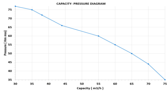
P013- 22D - KP500B2/20 22 HP Diesel Motopump Water Cooler - 3 Cylinders - 2 Stage High Pressure Suction 3" - Outlet 2,5"
