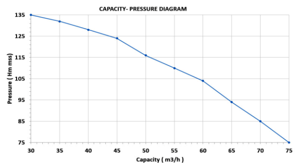
P015- 45D - KP500B4/40 P015 - 45 HP Diesel Motopump Water Cooler - 4 Cylinders 4 Stage High Pressure with Trailer Suction 4" - Outlet 3"
