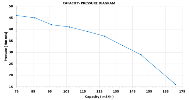
P013- 22D - KP500B2/20 22 HP Diesel Motopump Water Cooler - 3 Cylinders - 2 Stage High Pressure Suction 3" - Outlet 2,5"
