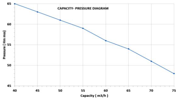
P012- 22D - SD325/20 22 HP Diesel Motopump Water Cooler - 3 Cylinders - 1 Stage High Pressure Suction 3" - Outlet 2,5"
